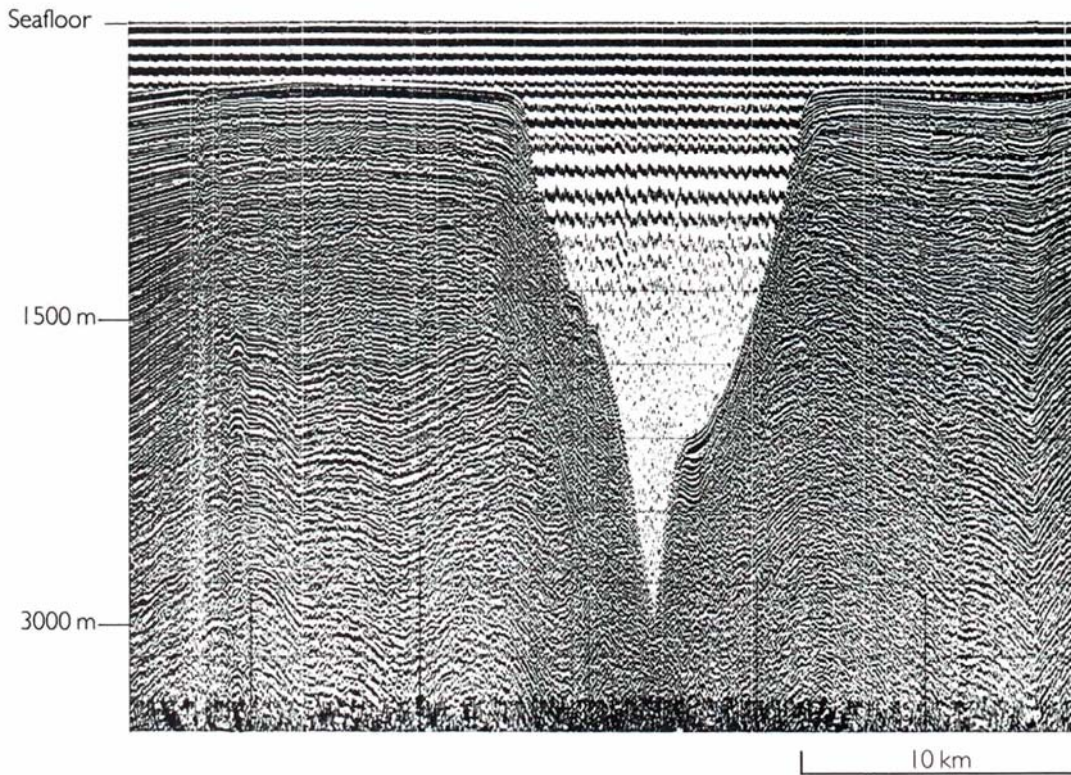
FIGURE 17.22 An echo-sounding profile of the Congo submarine canyon off the Republic of Zaire on the west coast of Africa. The bottom of the canyon at this point is about 3000 m below the seafloor of the continental shelf; at the top, the canyon is more than 10 km wide. The wavy lines below the seafloor surface are sound reflections from bedding planes in continental shelf sediments, somewhat deformed because of mild tectonic disturbance. (K. O. Emery, Woods Hole Oceanographic Institution.)
