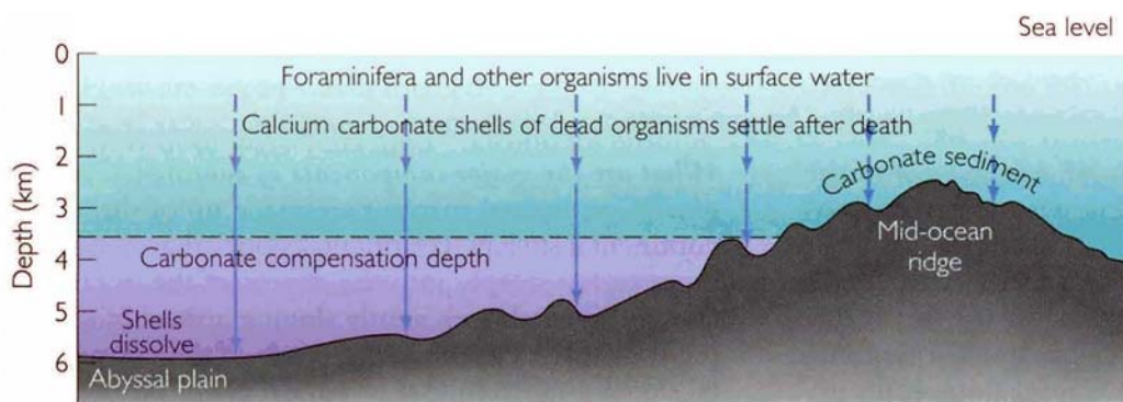
FIGURE 17.36 The carbonate compensation depth is the level in an ocean below which the calcium carbonate of foraminifera and other carbonate-shelled organisms that have settled from surface waters dissolves. As the shells of dead organisms settle into the deep waters, they enter an environment undersaturated in calcium carbonate and so dissolve.
