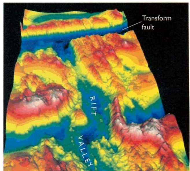
FIGURE 17.32 Above: A profile of the central rift valley of the Mid-Atlantic Ridge in the FAMOUS (French-American Mid-Ocean Undersea Study) area southwest of the Azores Islands. The deep valley, where most of the basalt is extruded, is faulted. (After ARCYANA, "Transform Fault and Rift Valley from Bathyscaph and Diving Saucer," Science , vol. 190, 1975, p. 108.) Right: Computer-generated image (based on data from multibeam sidescan sonar) of the Mid-Atlantic Ridge at about 31° south latitude reveals a 19-km-wide central valley studded with volcanic cones. The valley is bounded by mountains about 2000 m high. A transform fault intersects the valley at the top of the image. (K. C. Macdonald and P. J. Fox, "The Mid-Ocean Ridge," Scientific American , vol. 262, 1990, pp. 72–79.)
