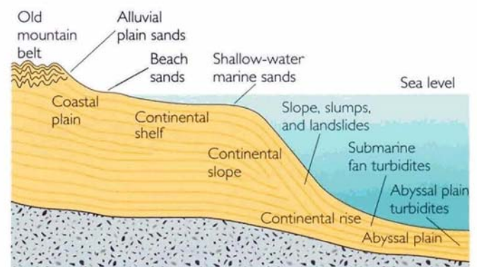
FIGURE 17.29 A profile of the Atlantic passive continental margin off southern New England. (After K. O. Emery and E. Uchupi, Atlantic Continental Margin of North America , American Association of Petroleum Geologists, 1972.)
