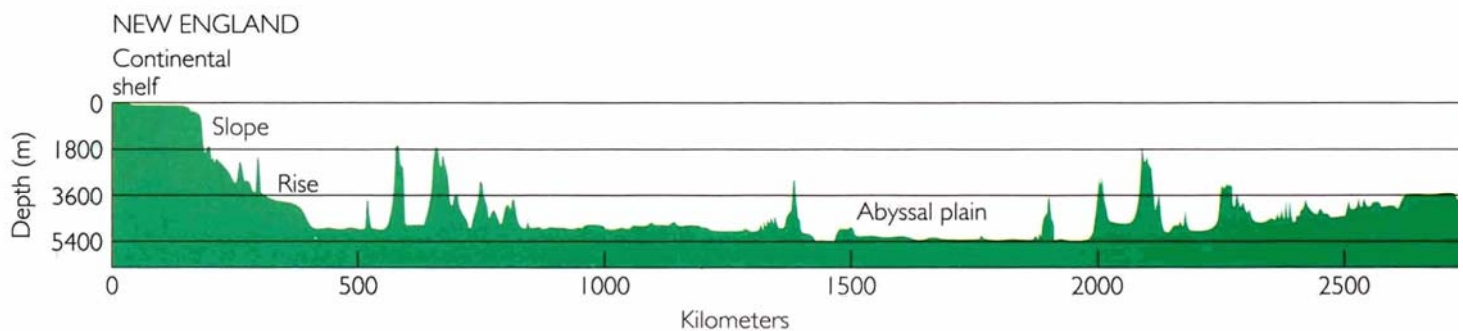
FIGURE 17.24 Topographic profile of the floor of the Atlantic Ocean from New England (left) to Gibraltar (right). (After B. C. Heezen, "The Origin of Submarine Canyons," Scientific American , August 1956, p. 36.)
