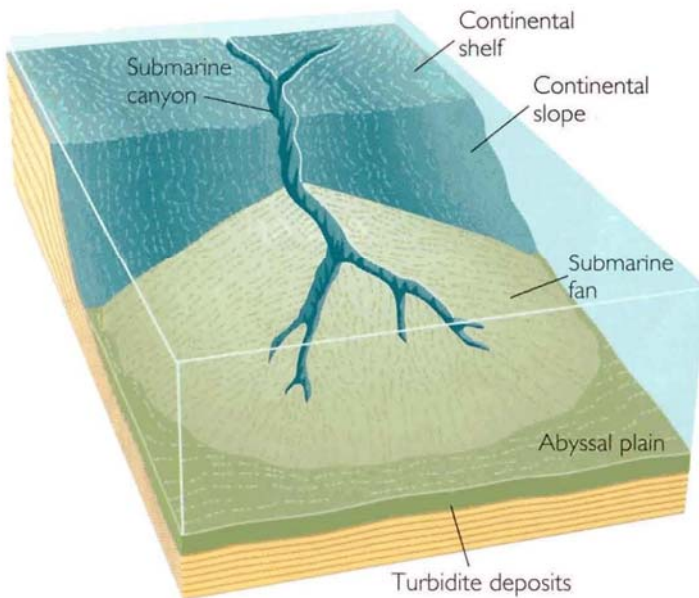
FIGURE 17.31 (a) Submarine canyons and fans are formed by turbidity currents that start on the continental shelf or slope and erode canyons in them, leading to channels on the fan. (b) Sandfall at the head of a submarine canyon at the edge of the continental shelf. These falls generate sandy flows, like turbidity currents, that lay down fans of sandy sediment at the foot of the continental slope. (U.S. Navy.)
