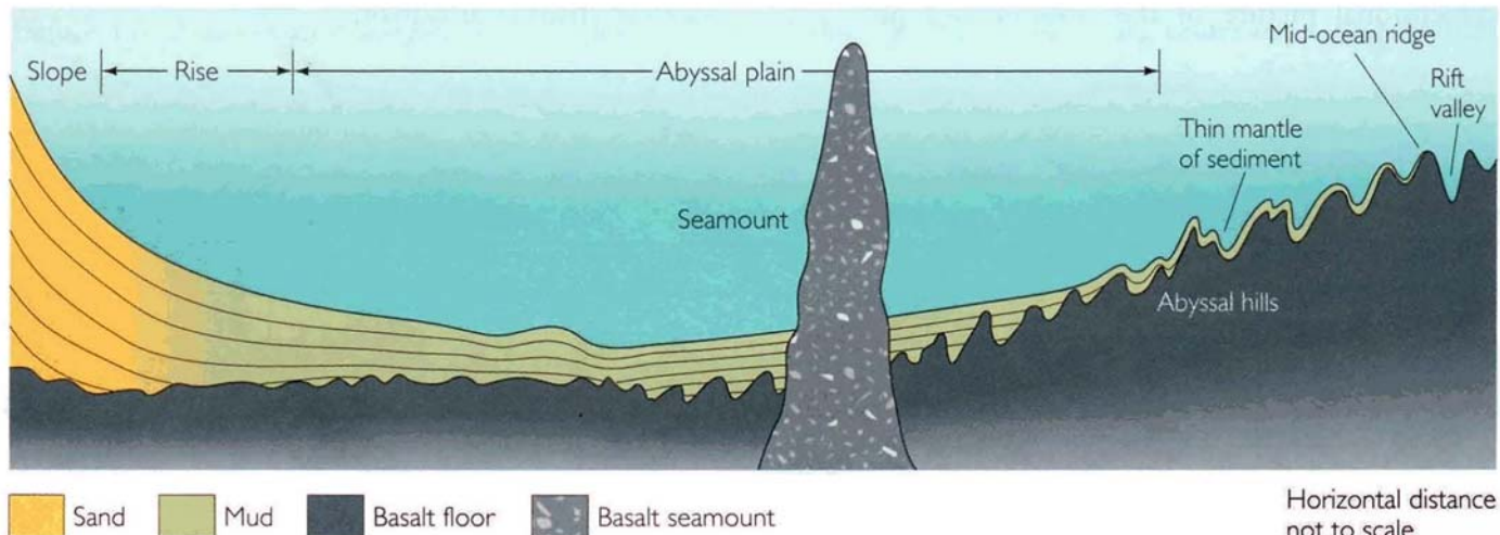
FIGURE 17.26 Profile from continental rise to Mid-Atlantic Ridge.
