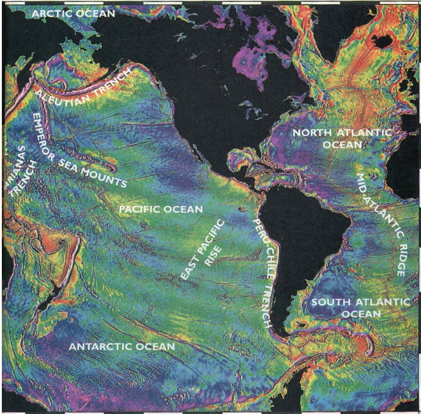
Marine gravity anomaly from satellite altimetry. (D. T. Sandwell and W. H. F. Smith/Geological Data Center, Scripps Institution of Oceanography, University of California, San Diego.)
