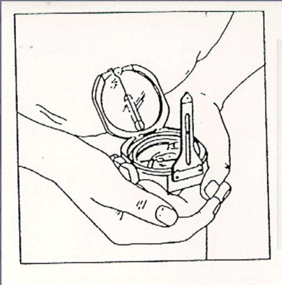
Brunton set for taking a bearing at waist height.
