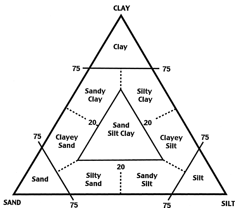
Figure 2. Ternary diagram for clastic textural groups (after Shephard (1954))
