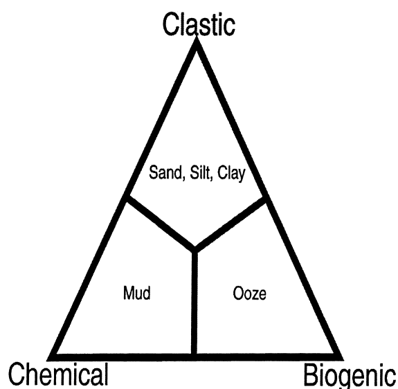
Figure 1. Ternary diagram illustrating principal names for classes of sediment.
