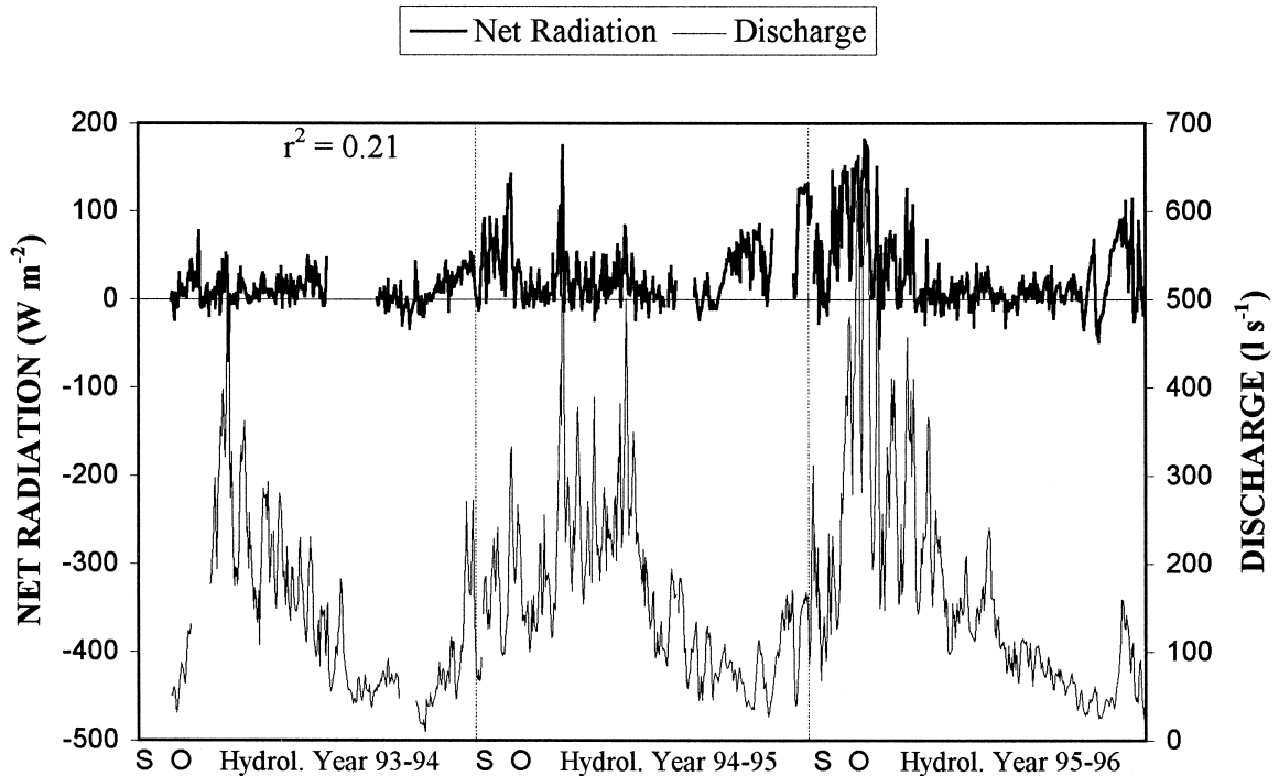
Fig. 4. Net radiation recorded by the automatic energy budget station at 5150 m a.s.l. and the daily discharge of the proglacial stream recorded at the gauging station at 4830 m a.s.l. (September 1993–August 1996).
