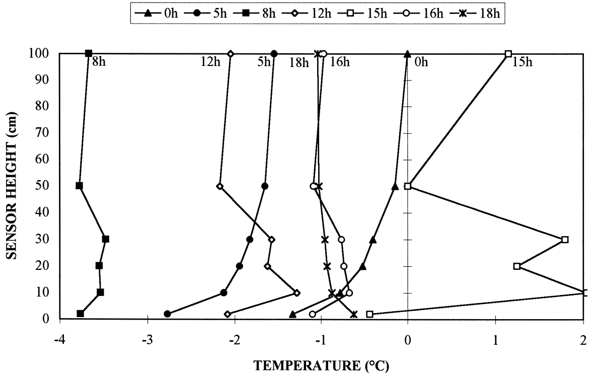
Fig. 5. Evolution of the vertical profiles of ventilated air temperature above the snow surface between 0 a.m. and 6 p.m. on March 3, 1997. At night, the profiles show a classical log–linear form, but during the day, a warm layer develops around 20–30 cm above the surface.
