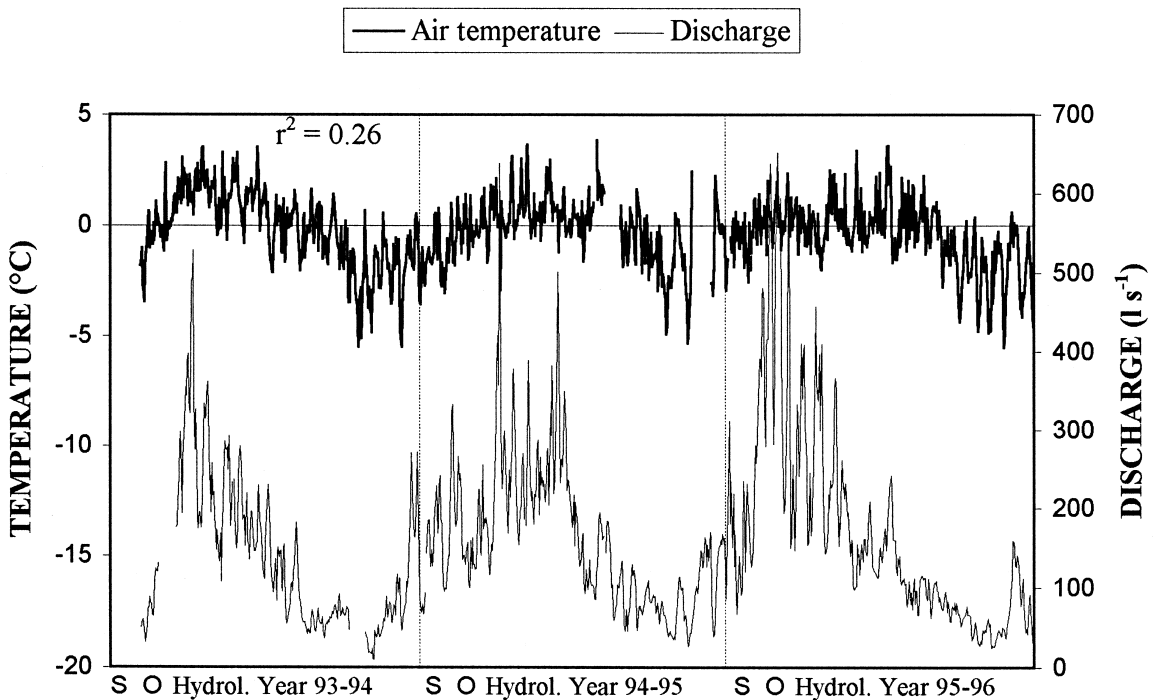
Fig. 3. Daily air temperature recorded by the automatic energy budget station at 5150 m a.s.l. and the daily discharge of the proglacial stream recorded at the gauging station at 4830 m a.s.l. (September 1993–August 1996).
