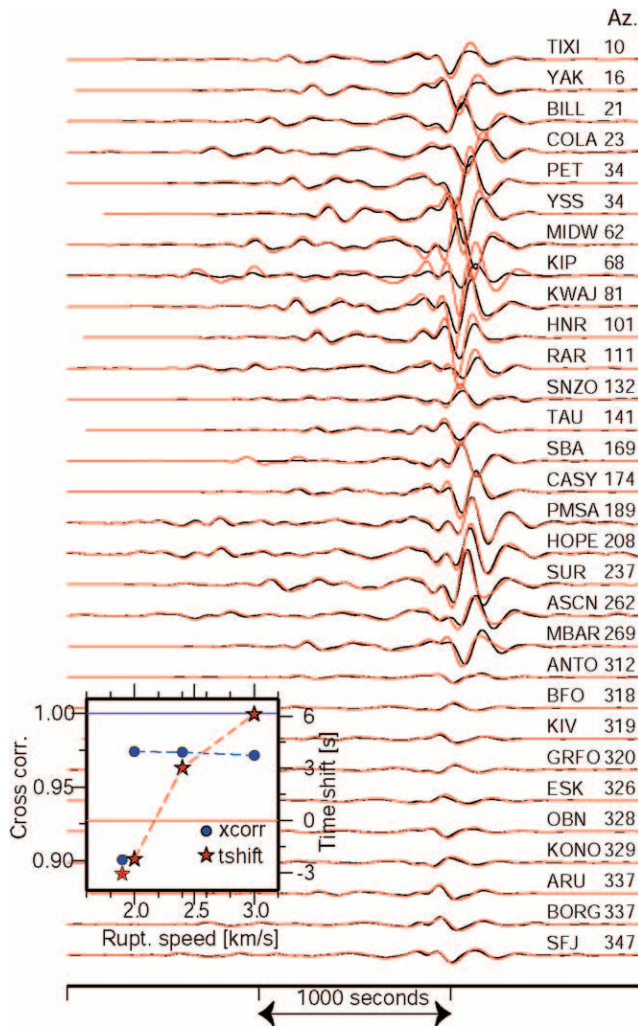
Figure 8. Fits to 100- to 500-sec bandpass-filtered waveform fits computed using a 3D SEM for the model with fixed rupture velocity of 2.5 km/sec (Fig. 7c). The seismograms are 30°–100° distance and are sorted by azimuth and aligned on the Rayleigh wave (3.8 km/sec phase velocity). The inset shows the cross-correlation values (blue circles) and time shifts (red stars) of the Rayleigh waves for the fixed rupture velocity models of 1.5, 2.0, 2.5, and 3.0 km/sec.
