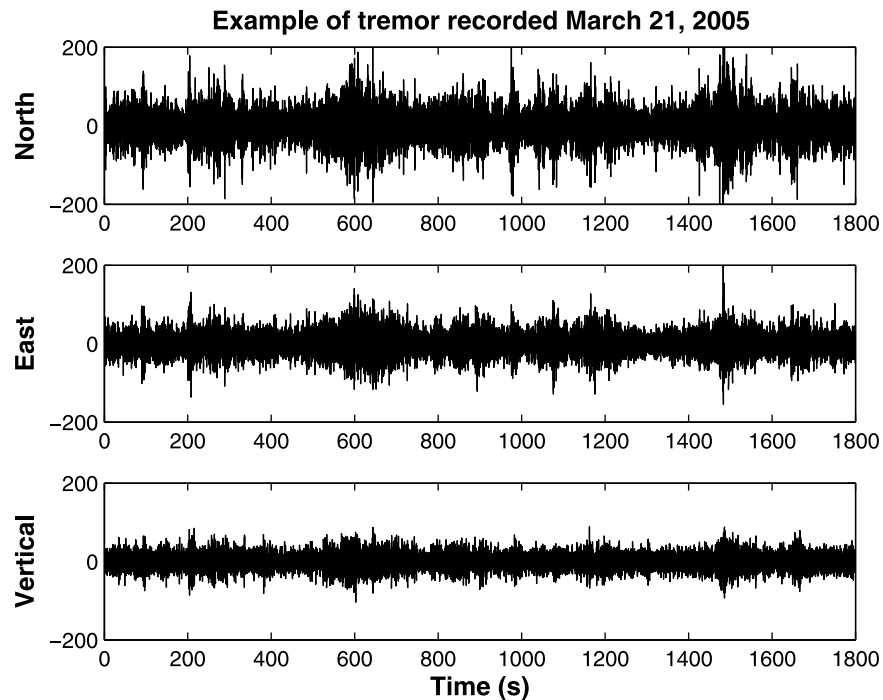
Figure 2. Example tremor seismogram. This is from an NVT episode recorded at the station TONA approximately 200 km from the trench [Pérez-Campos et al. , 2008]. The northern component is clearly larger than the eastern component. The vertical component is clearly the smallest component. This was typical for the tremor measured in this study.
