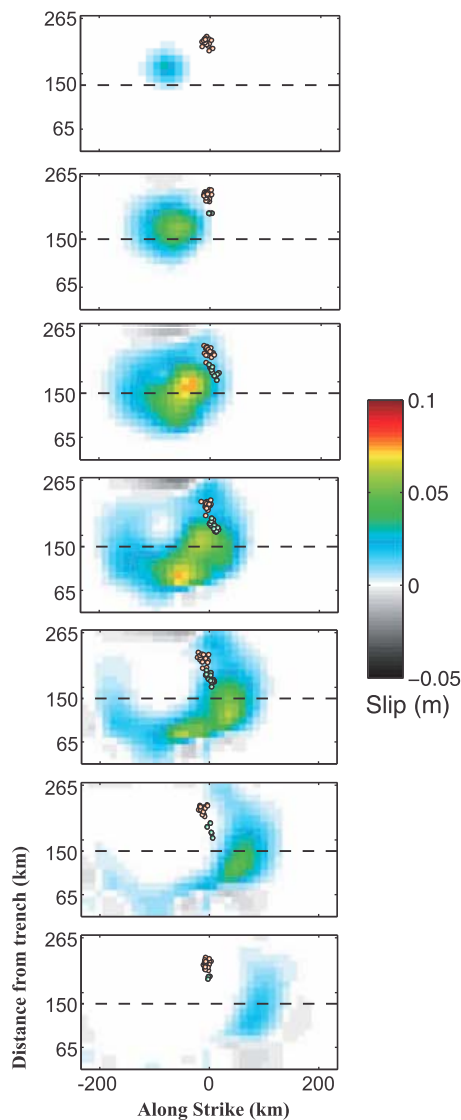
Figure 7. NVT epicenters from this article and the 2006 SSE slipping front from Radiguet et al. [2011]. The downdip, high-energy NVT (orange dots) and the updip, low-energy NVT (green dots) and the inter-episode NVT (gray dots) correspond to Figures 1, 3, 5, and 6. The plots are in chronological order starting January 30, 2006 at the top and ending 350 days later January 15, 2007 at the bottom. Each plot contains 50 days of NVT and slip.
