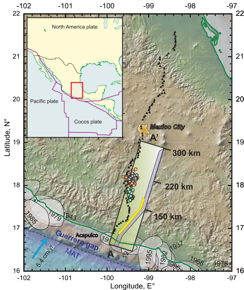
Figure 1. Map of the NVT epicenters (dots) found in this study. The orange dots are the down-dip epicenters. The gray dots are the inter-episode epicenters. The green dots are the up-dip epicenters. Inset shows the setting of the study area (red rectangle). The black triangles are the locations of the MASE seismometers. The profile A-A' is the same profile shown in Figures 3–5. The shape of the slab (purple) and the location of the 2006 SSE (yellow) are shown in the horizontal cartoon for clarity, but the cartoon should actually be vertical, extending into the Earth from the MASE array. The distance markers are measured from the Middle American Trench (MAT). The dashed line, MAT, is the Middle America Trench. Shaded regions along the coast are the rupture areas of the most recent large subduction thrust earthquakes annotated with its year of occurrence. Blue arrow indicate the convergence velocity vector according to the NUVEL 1 A model [DeMets et al. , 1994].
