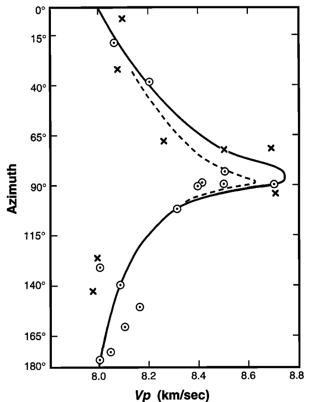
Figure 2. Variation of seismic V_p velocity with azimuth for refraction surveys near the Mendocino fracture zone area off California. The E-W fast direction parallels the fracture zones in the region and was the first evidence that olivine a axes may align parallel to spreading. Circles, Mendocino area; crosses, Maui area; dashed curve, model for Mendocino; solid curve, model for both areas combined. (Reprinted with permission from Nature Copyright 1964 Macmillan Magazines Limited.) [ Hess , 1964].
