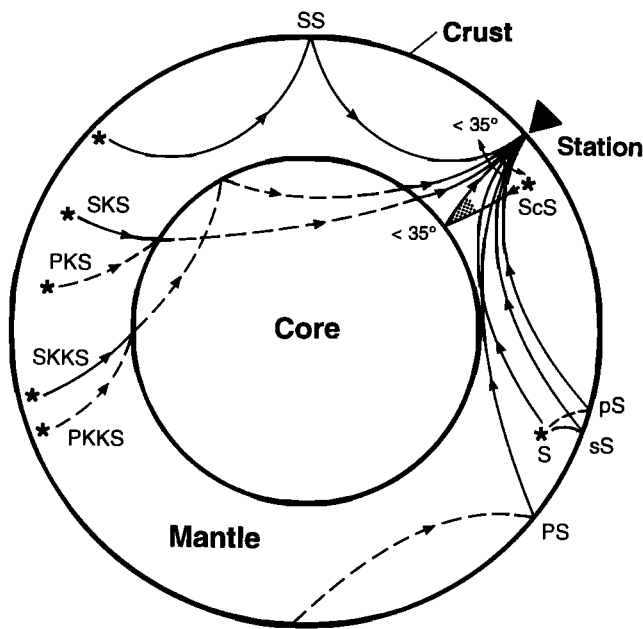
Figure 6. Phases that have been used for shear wave splitting studies. The shear wave window of 35^\circ at the surface and at the core-mantle boundary ensures phases with smaller incidence angles will yield linear S wave particle motion for isotropic propagation (see glossary). Solid lines are S path segments, dashed lines are P path segments, and stars are earthquake sources.
