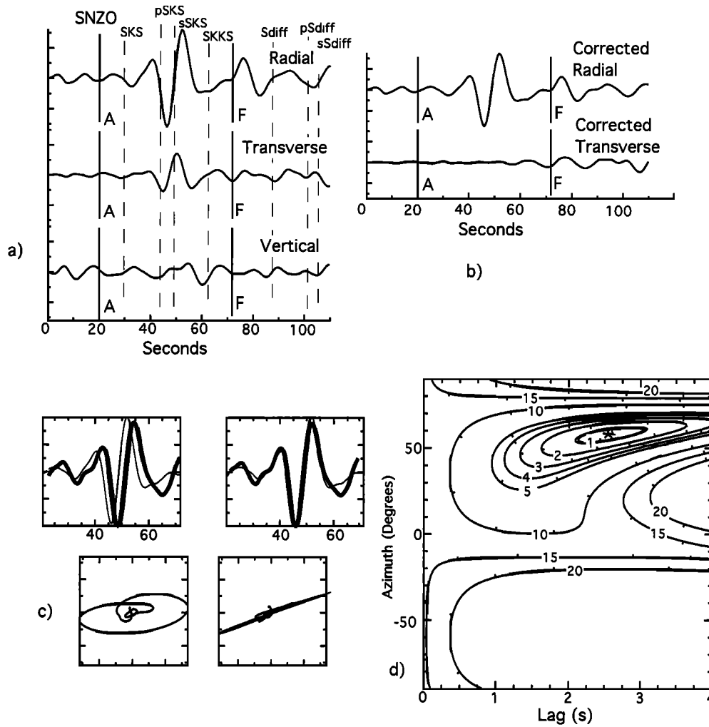
Figure A4. Example of a good shear wave splitting measurement using the method of Silver and Chan [1991] along with the diagnostic plots from station SNZO, New Zealand [ Marson-Pidgeon and Savage , 1997]. (a) Original (filtered) radial, transverse, and vertical component seismograms, with scale set by the radial component amplitude. Predicted phase arrivals are displayed along with the time interval (between A and F) used to make the measurements. (b) Corrected radial and transverse components. Note that the corrected transverse component has been minimized. (c) (top) superposition of fast and slow (bold) components uncorrected (left) and corrected (right). Note the similarity of the pulse shapes. (bottom) Corresponding particle motion diagrams. Note that the elliptical particle motion becomes linear when corrected. (d) Contour plot of the energy on the corrected transverse component showing the minimum value (star) along with the 95% confidence region (double contour) and multiples of that contour interval.
