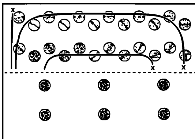
Figure 5. Model of a convection cell with stereographs of a axes pole figures describing the anisotropy throughout the cell. Bold line is path followed to reach position X. Dashed line, located at 150 km depth, separates weak anisotropic olivine aggregate above from more rigid isotropic material below, which is designed to correspond to a transformation from olivine to spinel/perovskite. Note the wide variation of a axis alignments throughout the upper cell. From Chastel et al. [1993, problem A, Figures 11 and 14].
