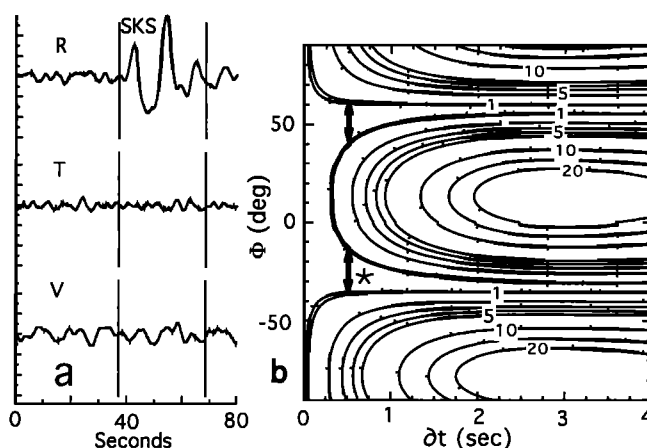
Figure A5. Example of a null measurement at station CCY in the Rocky Mountains [after Savage et al. , 1996b]. (a) Seismograms rotated to (top) radial, (middle) tangential, and (bottom) vertical orientations. The SKS phase used in the measurement lies between the solid lines. (b) Contour plot of the energy on the tangential component for seismograms corrected to the given azimuths of \phi or lag \delta t . The 95% confidence interval is the double contour, with multiples of this interval labeled. The elongate 95% confidence region is typical of a null measurement, in which any amount of splitting is allowed, provided that the fast axis occurs at azimuths equal to the back azimuth or the back azimuth minus 90^\circ . Arrows show the allowed azimuth ranges of fast axes of anisotropy at 0.5 s splitting.
