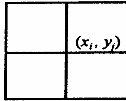
Fig 1a: Node (x_i, y_j) , surrounded by four squares.
